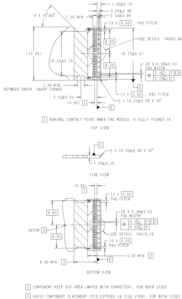
Figure 3-19: OSFP module pc board (card-edge)
