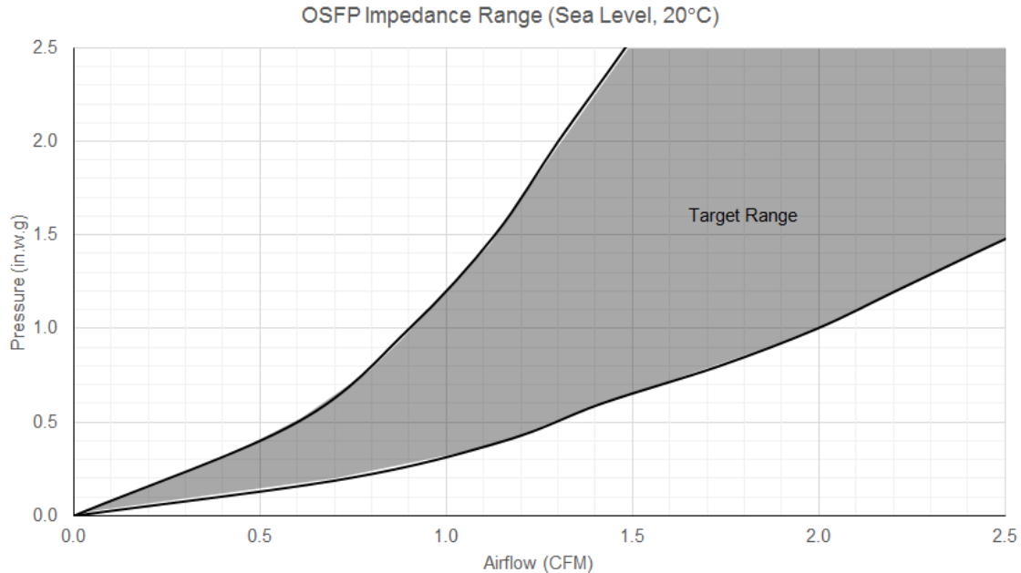
Figure 8-1: Target range of impediment to airflow of an OSFP module (20C, Sea Level)
