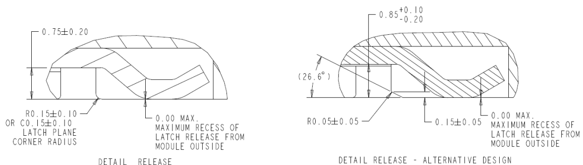
Figure 3-25: Latch plane corner radius and release details
