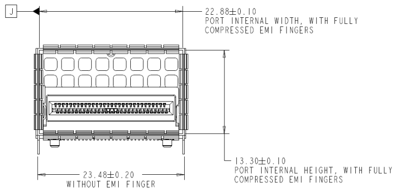
Figure 4-4: Port internal width and height
