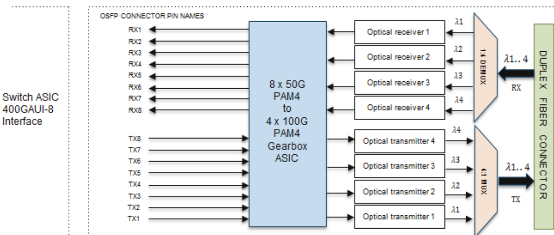
Figure 10-4: Block diagram for 400G-FR4
