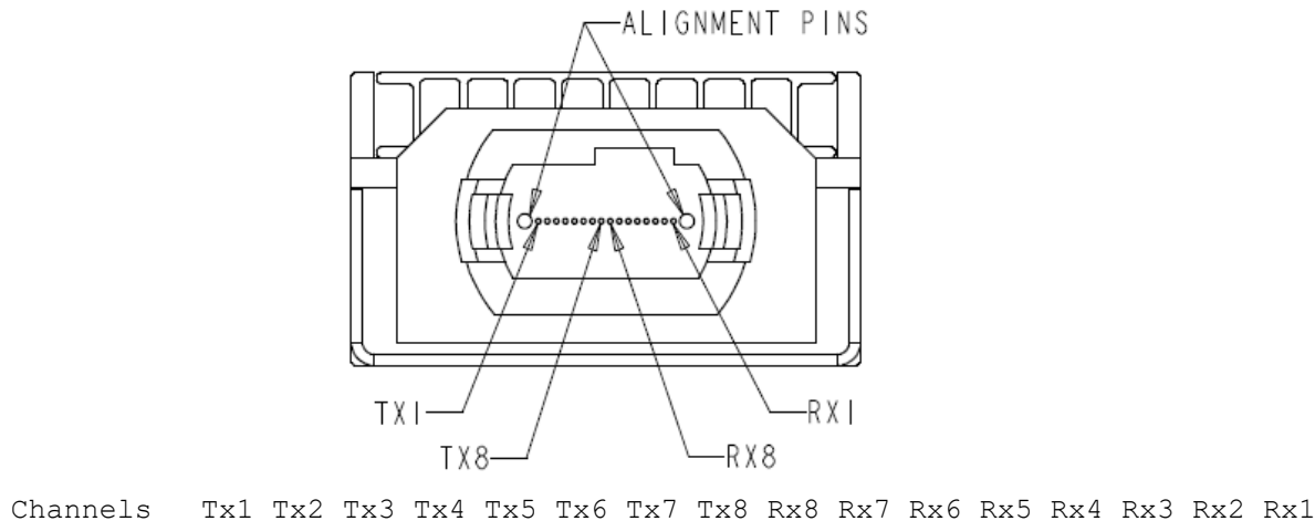
Figure 10-18: Optical receptacle and channel orientation for MPO-16 connector
