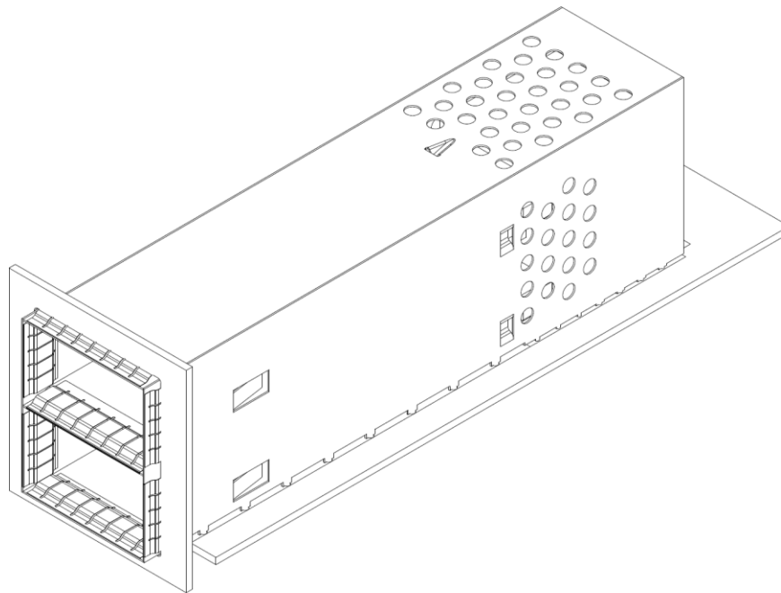
Figure 5-1: Stacked SMT 2x1 cage with host PCB and the panel
