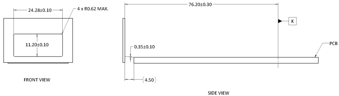
Figure 9-19: Bezel cutout for the OSFP-RHS cage
