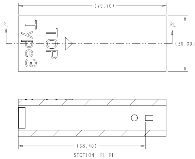
Figure 8-4: Impedance test jig for Type 3 OSFP
