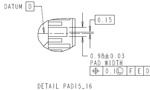
Figure 3-21: OSFP card-edge, detail of power pad (pads 15/16)
