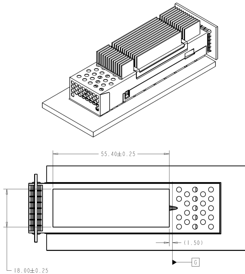
Figure 4-12: OSFP with a riding heatsink (above) and cutout on the cage for a riding heatsink in OSFP (bottom)
