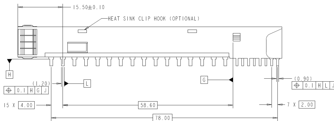
Figure 9-13: Cage positioning pins and forward stop
