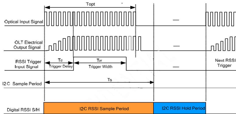
Figure 6 Timing Parameter Definitions in RSSI Trigger
