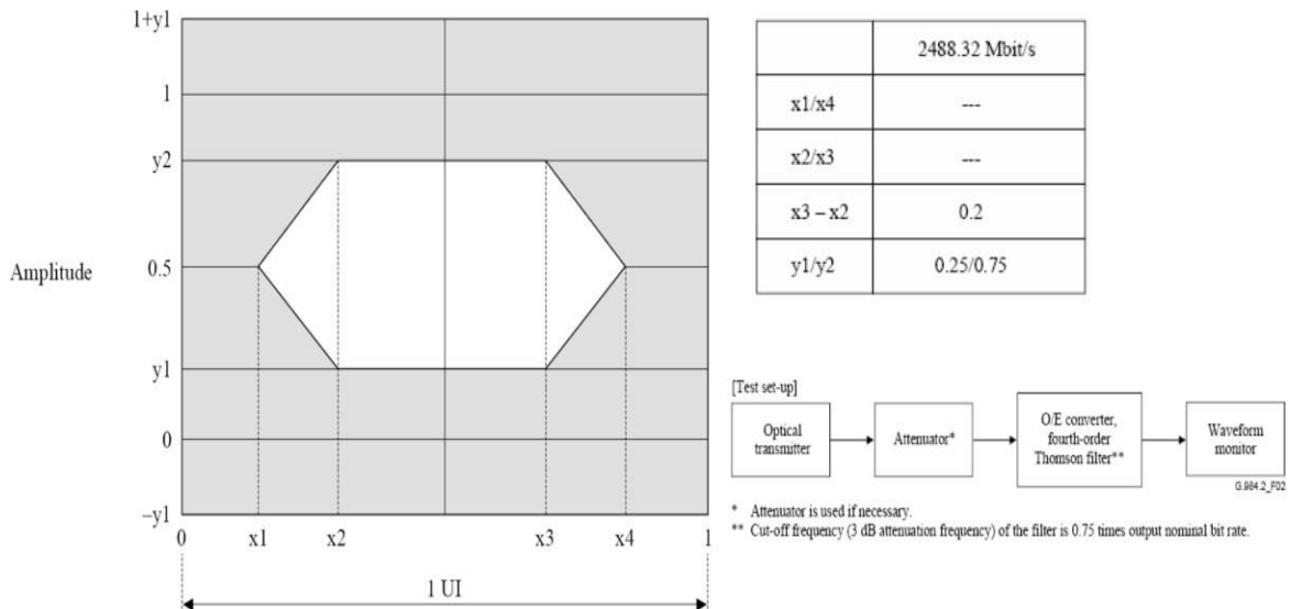
Figure 2 GPON Transmitter Eye Mask Definitions
