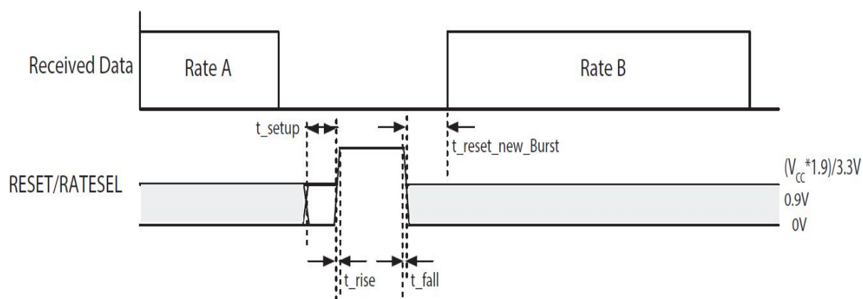
Figure 4 Reset/RateSel Timing Diagram
