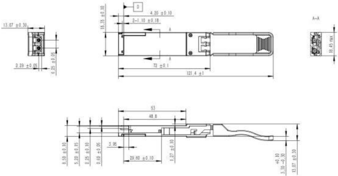
Figure 2. Mechanical dimensions
