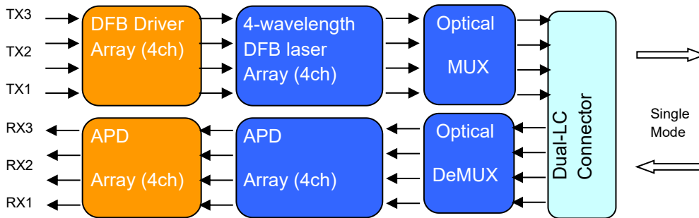
Figure 1: 40Gb/s QSFP ZR4 Transceiver Block Diagram
