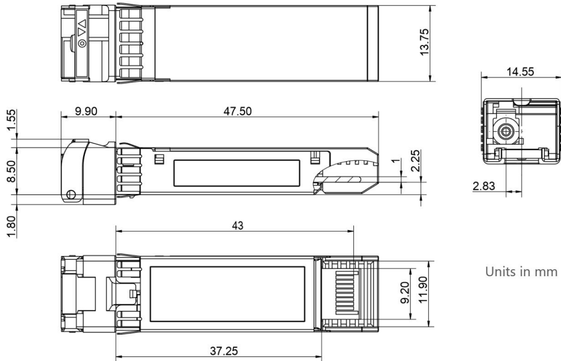
Figure2. Mechanical Outline
