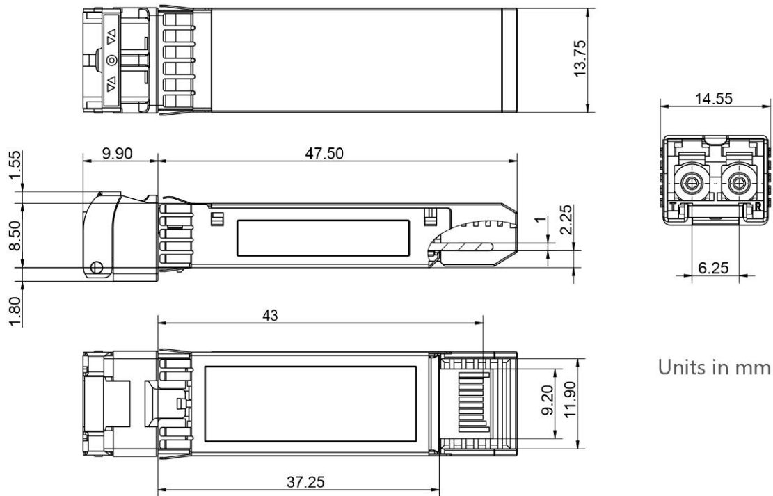
Figure2. Mechanical Outline
