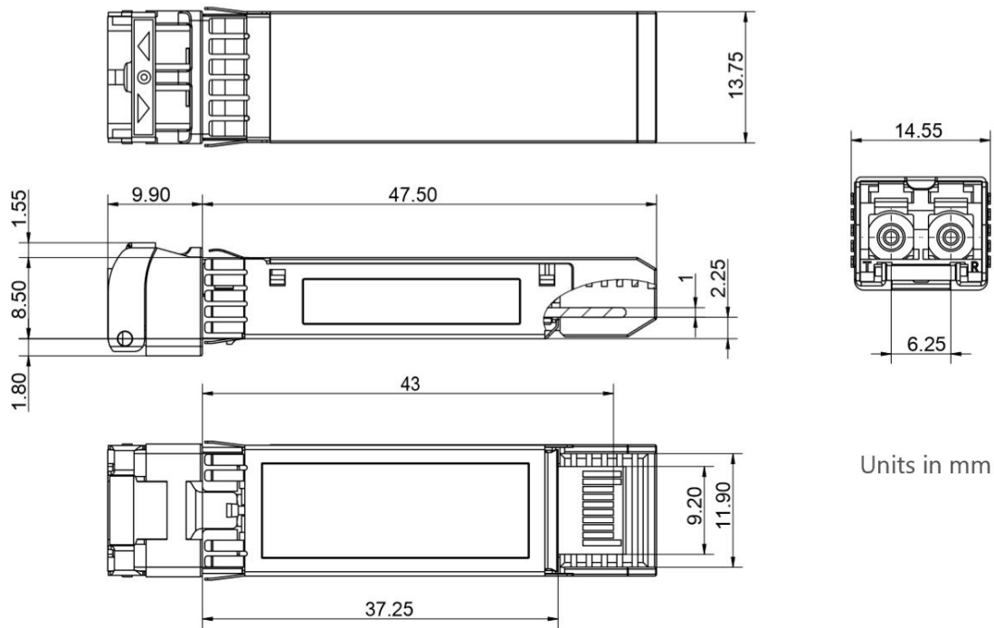
Figure2. Mechanical Outline
